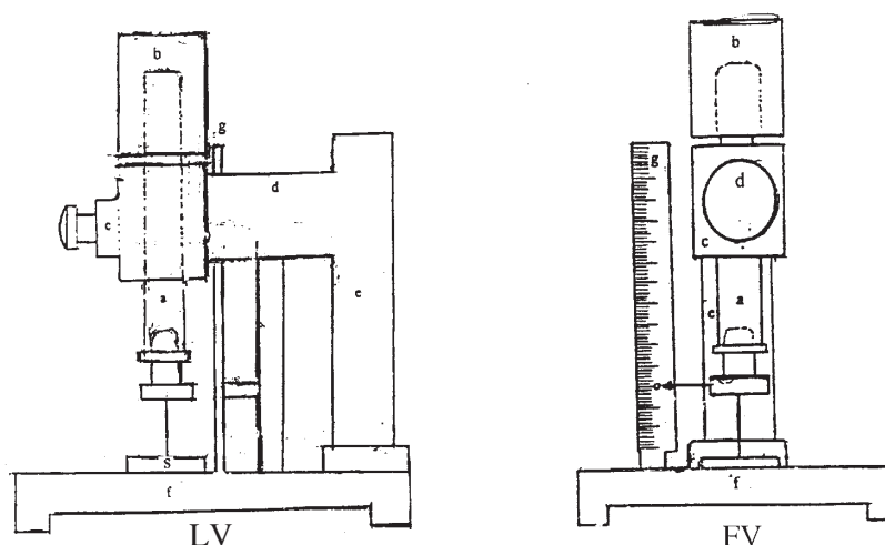
Figure 1. Lateral View (LV) and Front View (FV) of the setting time instrument (ISO 4823. 1984).
