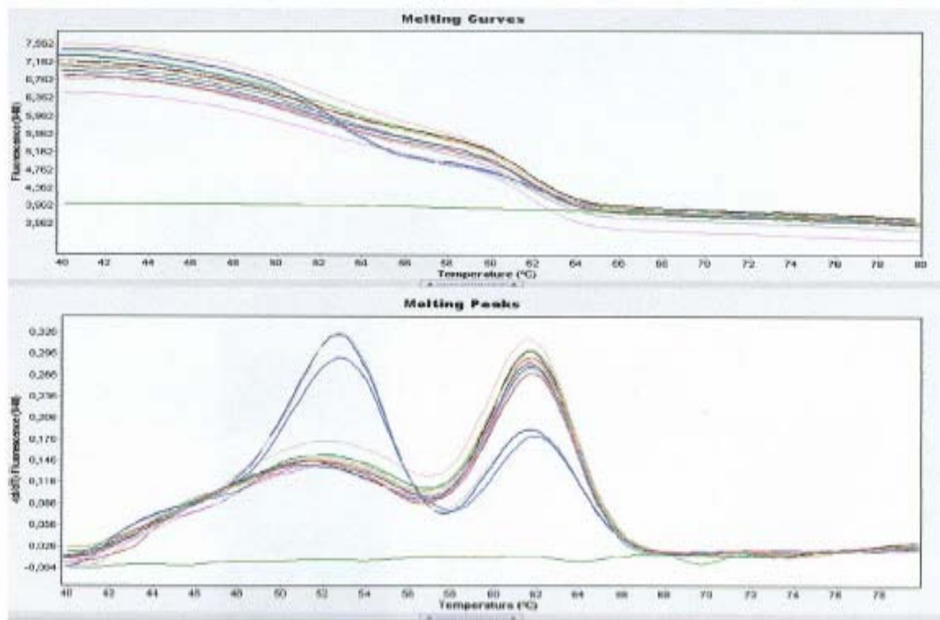
Figure 4. Typical example of melting curves and melting peaks used to genotype C677T MTHFR gene mutation. The probe and positive control that was used provided by the manufactures. Melting peak temperatures obtained from a derivative of the melting curves are 62.0 °C for homozygous wt (C/C), 52.4 °C and 62.0 °C for heterozygous (C/T). No homozygous mutant type (T/T) was observed.
