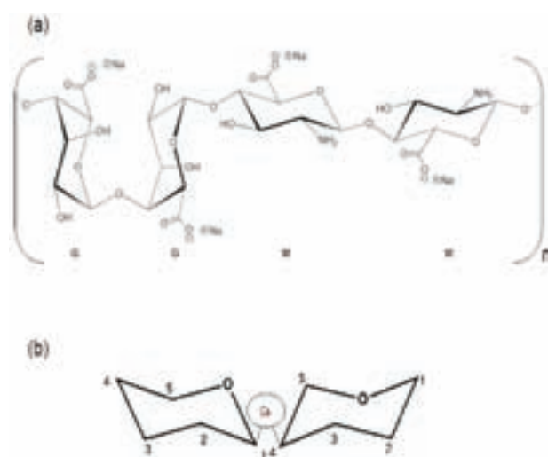
Figure 2. Scheme diagram (a) alginate expressed as Guluronat acid (G unit) Manuronat acid (M unit) forming (b) cross-linked at C1 and C4. 12
